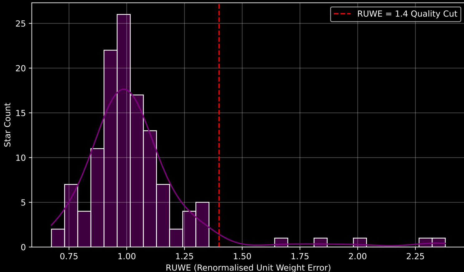
GAPOGEE DR17 Field [010+02] RUWE Distribution (n= 125)
