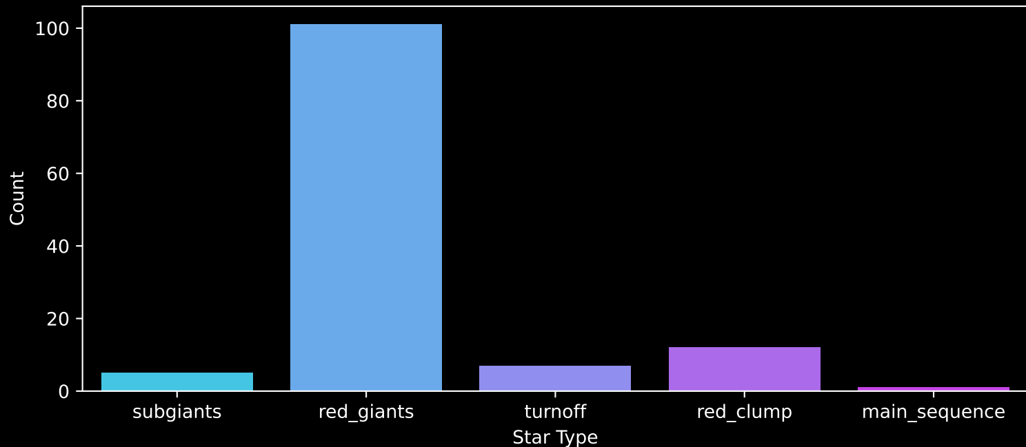
APOGEE DR17 Field: [010+02] Count plot of Star Type
