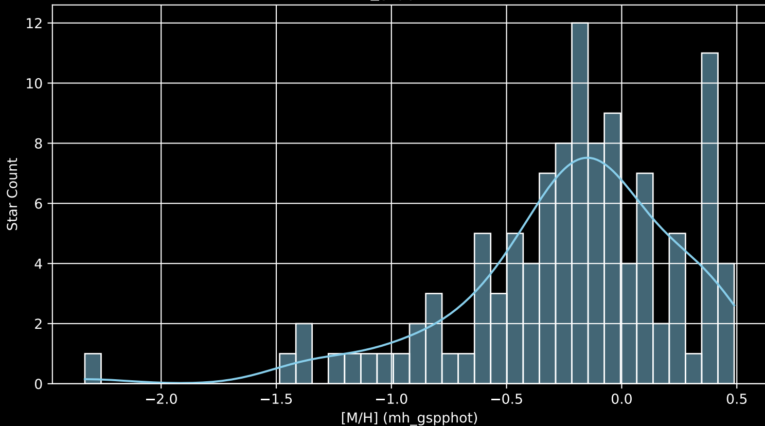
APOGEE DR17 Field: [010+02 [M/H] (mh_gspphot) (n= 111)
