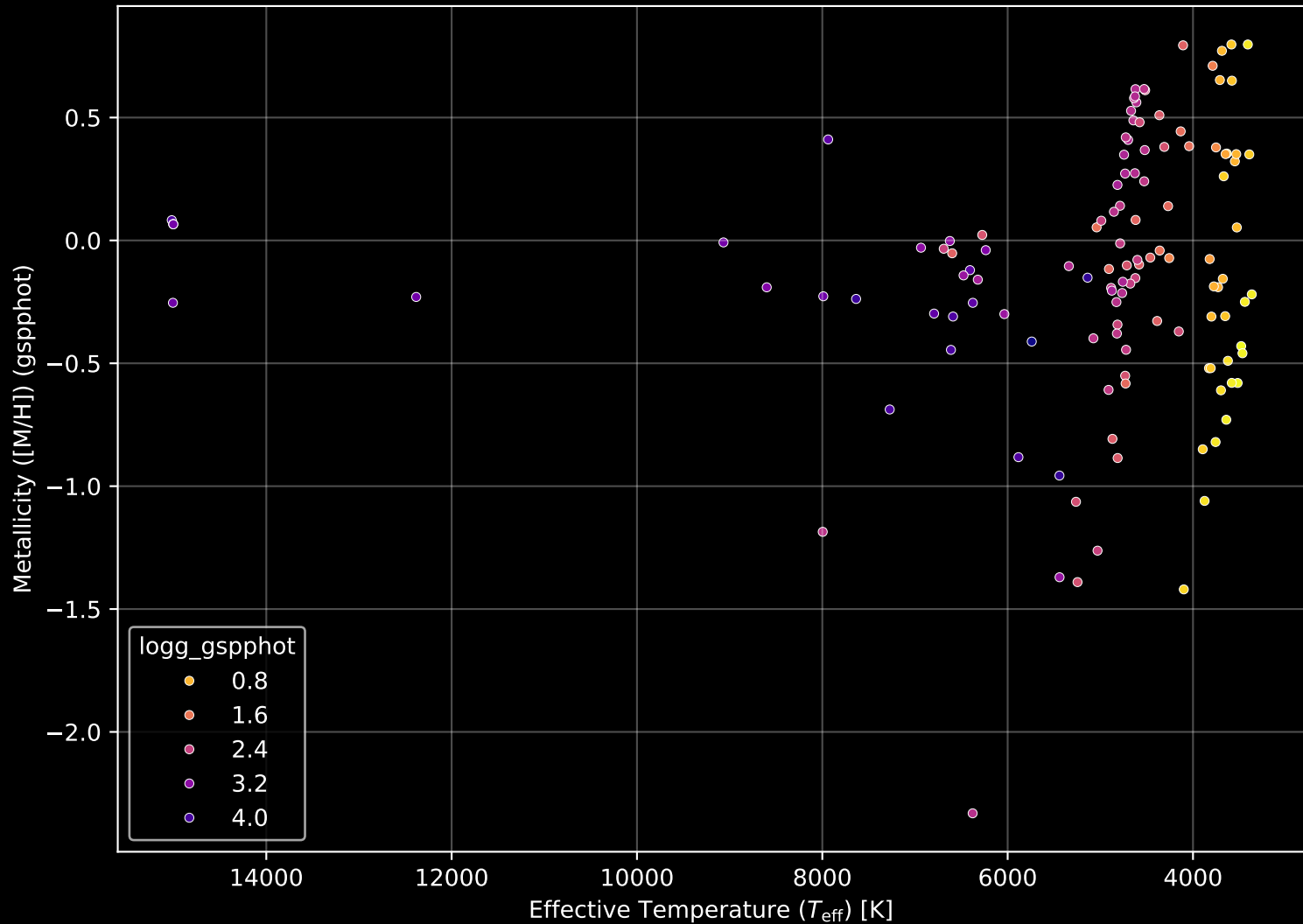
APOGEE DR17 Field: [010+02] Stellar Population Parameters (n= 126)
