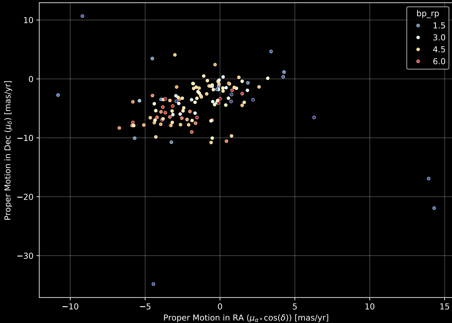
APOGEE DR17 Field: [010+02] Proper Motion Diagram (n= 126)
