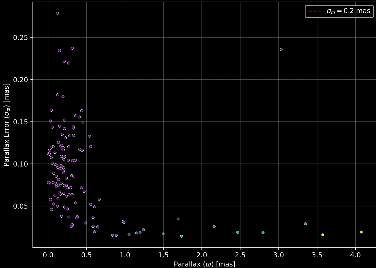
APOGEE DR17 Field: [010+02] Parallax Quality (n= 126)
